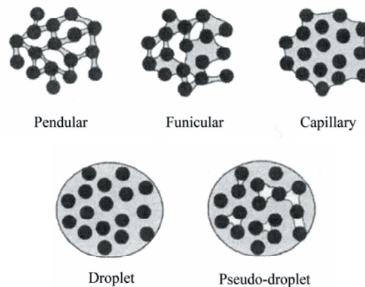
Figure 1: Spatial agglomeration structures. The different formal spatial structures of liquid-bound agglomerates depending of liquid saturation (Iveson et al., 2001a).
