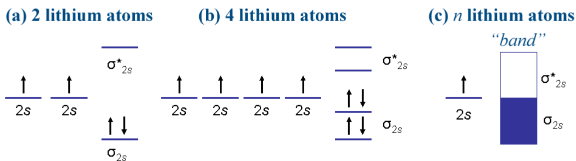
Figure 2-19: The energy levels for the molecular orbitals for lithium metal (a) Two lithium atoms together create two molecular orbitals. (b) Four lithium atoms together create four molecular orbitals. (c) n lithium atoms together create n molecular orbitals. When the number of atoms is large, the energy levels of the molecular orbitals created a continuous energy band .
