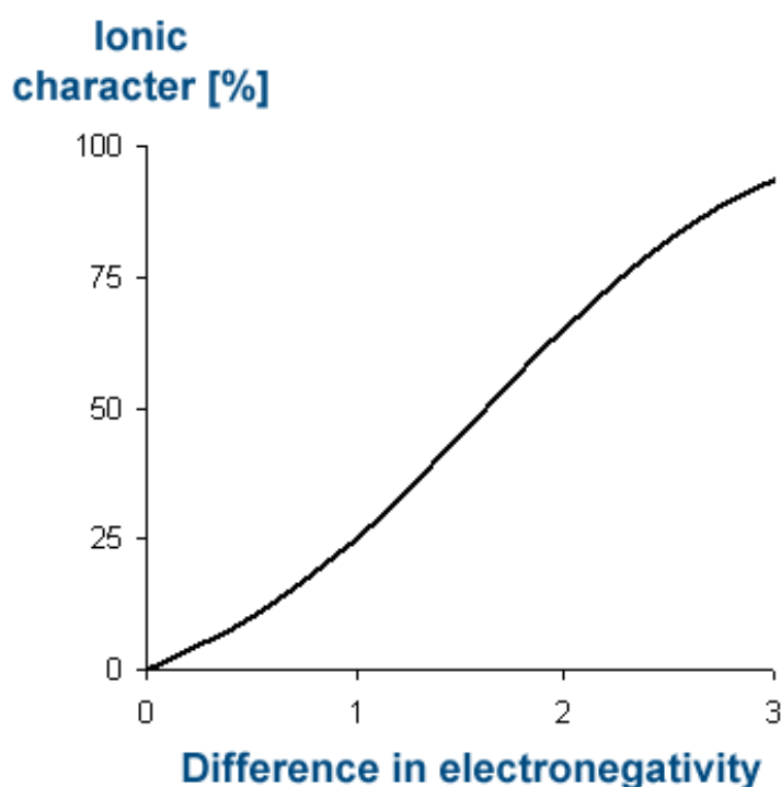
Figure 2-24: Ionic character
