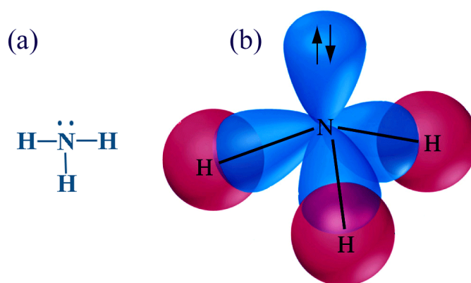
Figure 2-16: sp^3 -hybridization in \text{NH}_3
