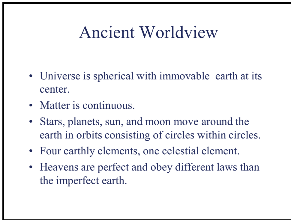
Figure 6: Ancient worldview.
