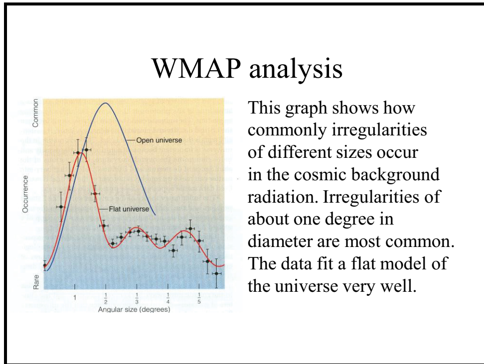
Figure 9.9 WMAP analysis
