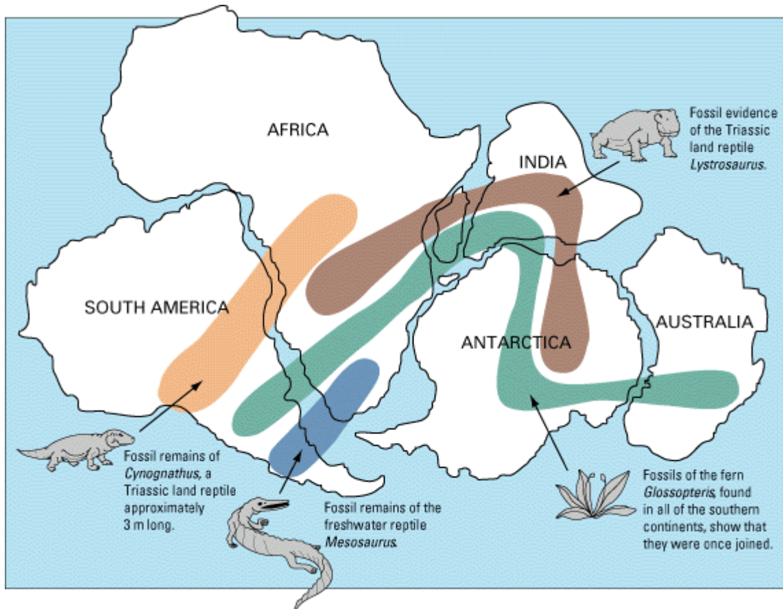
Figure 11.4 Fossil distribution
