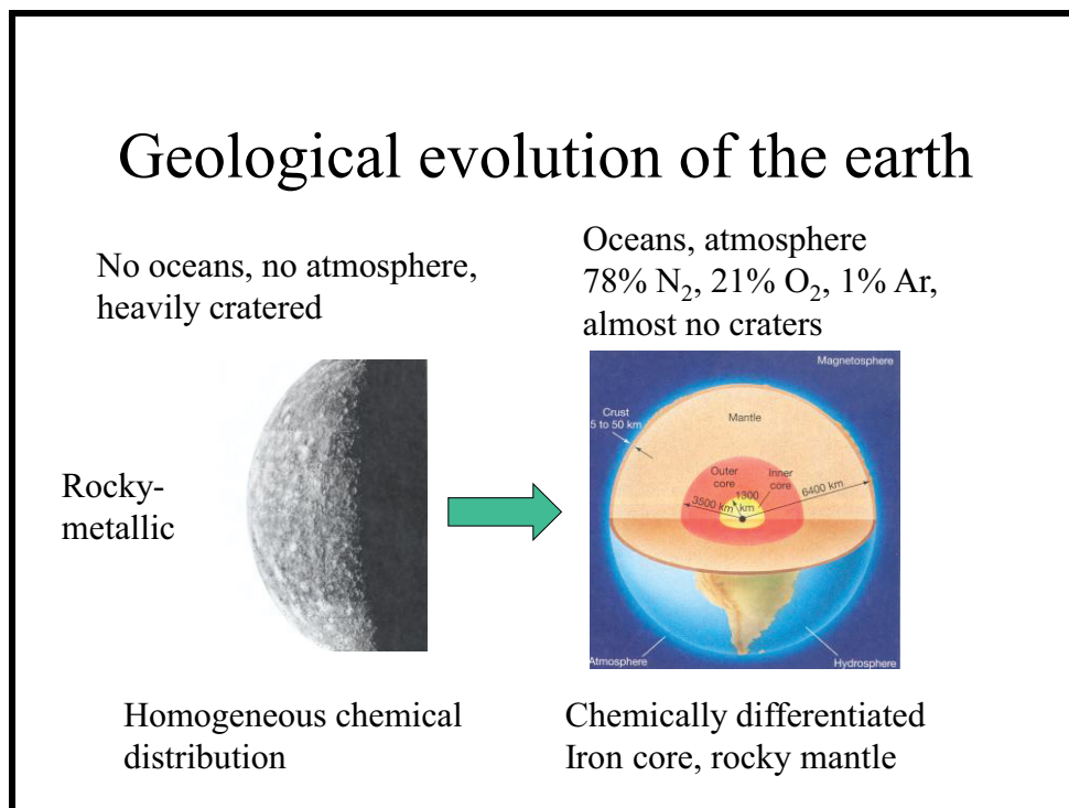
Figure 11.3 Geological evolution
