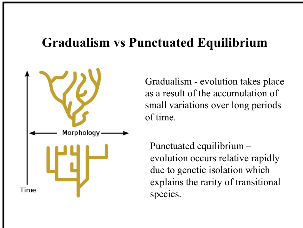
Figure 4 Punctuated Equilibrium
