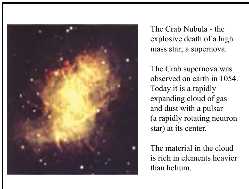
Figure 10.13 Crab Nebula
