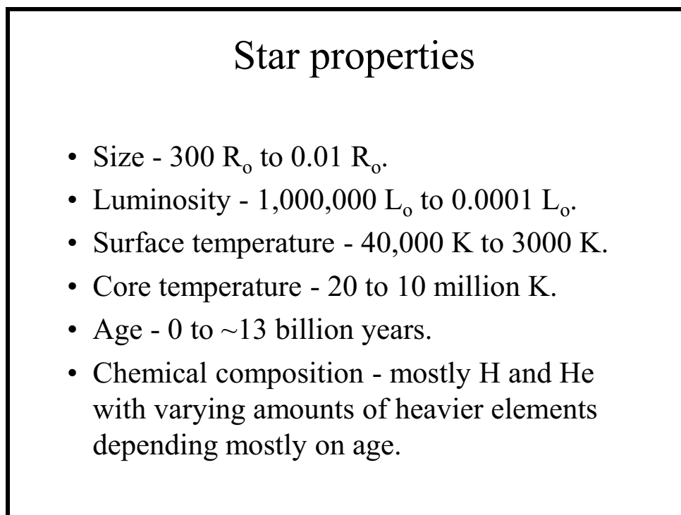
Figure 10.7 Star properties
