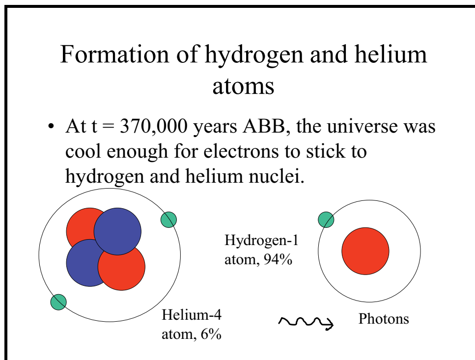
Figure 8.3 Atoms
