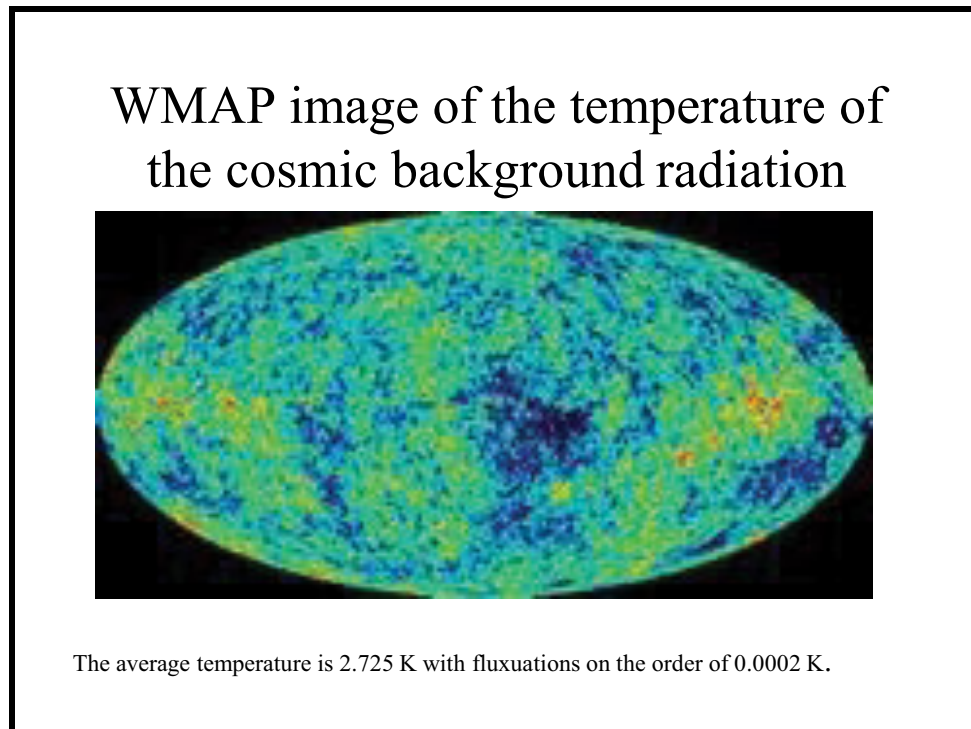
Figure 9.2 WMAP image
