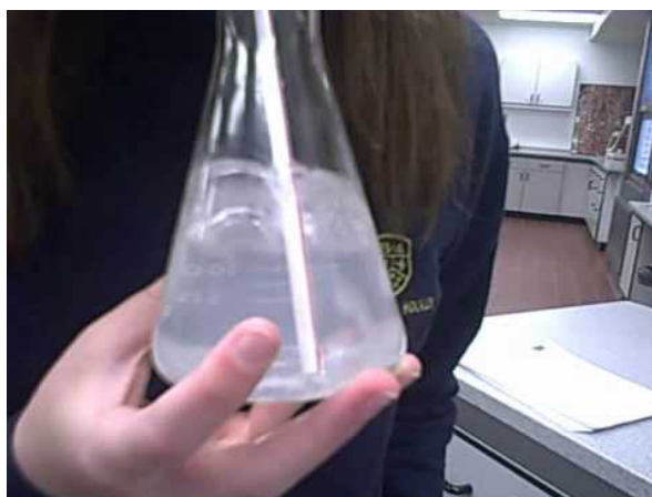
Blowing into limewater, showing that breath contains flue gas [Wiscolt, YouTube]
