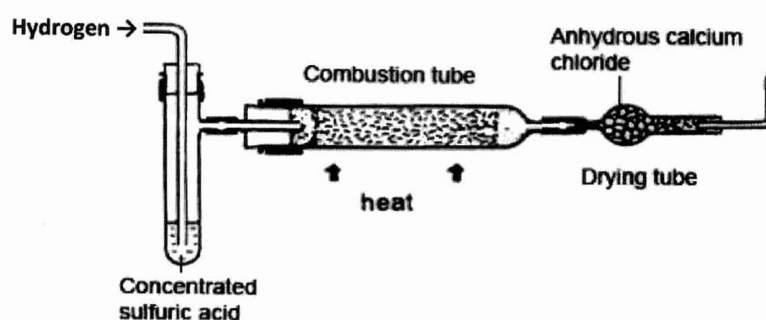
Apparatus for heating cupric oxide in hydrogen and weighing the water formed by absorbing it in anhydrous calcium chloride
