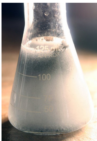
Hydrogen peroxide solution decomposing into bubbles of oxygen in the presence of a black catalyst (manganese dioxide) [Chemistry Land CHM130LL]
