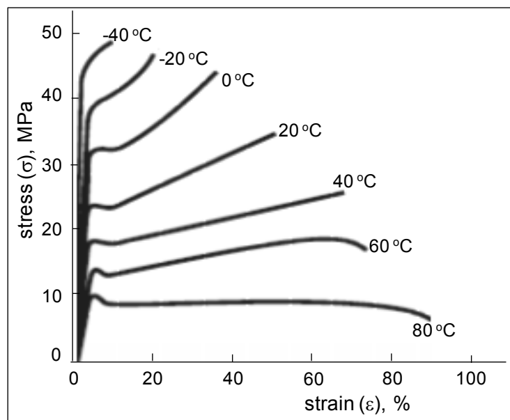
Figure 6.7 Stress-strain curves for HIPS at a range of temperatures from -40 °C to 80 °C (tests conducted at 2 mm/min cross-head speed) (source: Ehrenstein (2001, p182))
