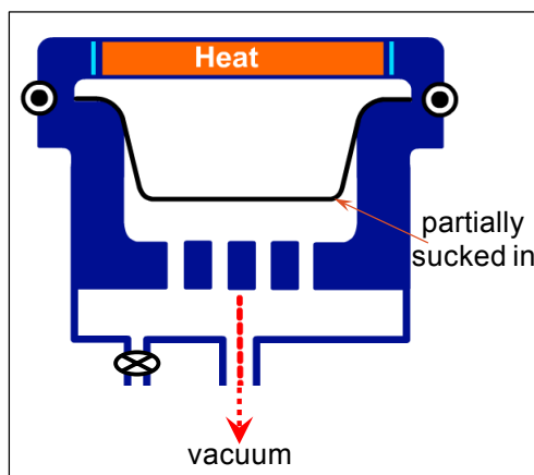
Figure 3.43 Illustration of vacuum forming
