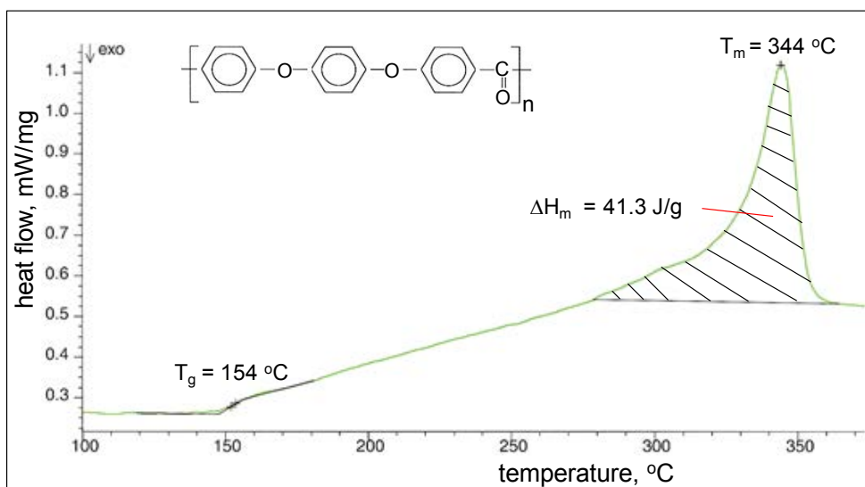
Figure 4.14 DSC trace for a PEEK specimen (source: Netzsch GmbH)
