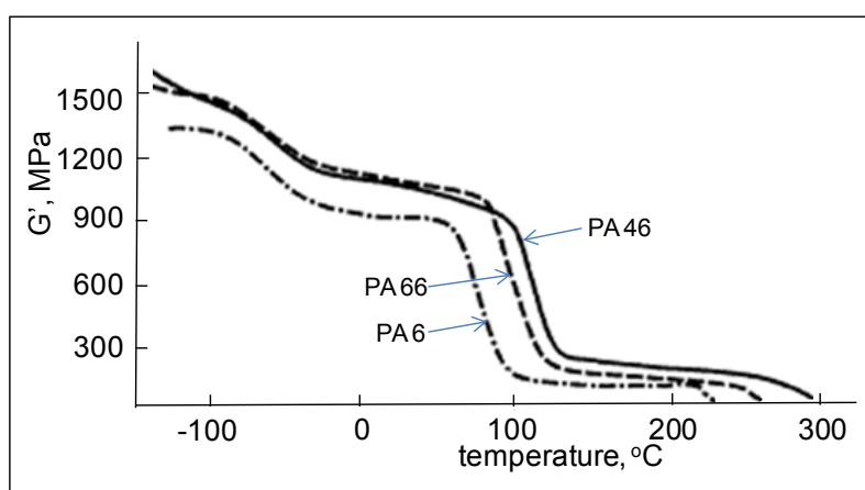
Figure 7.19 Storage modulus ( G' ) vs. temperature for polyamides. The tests are conducted in torsion at 1 Hz frequency and 3 °C/min heating rate (source: Ehrenstein 2004, p279)
