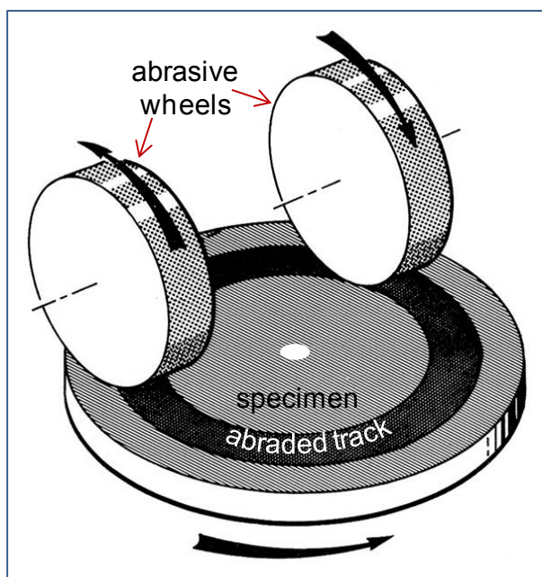
Figure 6.31 Taber abrasion set up (source: Taber Industries)
