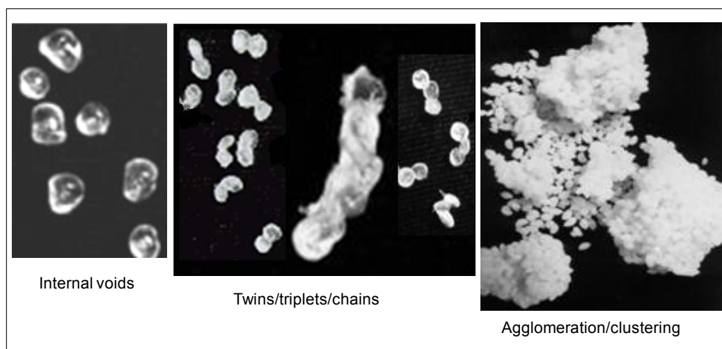
Figure 2.4 Various types of defects in pelletisation: fast cooling resulting in voids and slow cooling in agglomeration of pellets from twins to large clusters (source: http://www.er-we-pa.de/public_html/Company/pubs/EP_defects.html )
