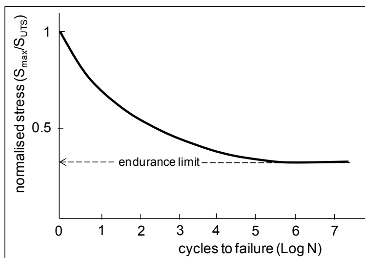
Figure 6.30 S-N curve
