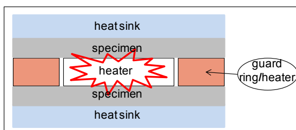
Figure 7.33 Guarded hot-plate set up
