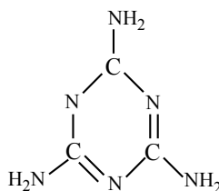
Figure 3.50 Melamine (a cyclic amino compound)
