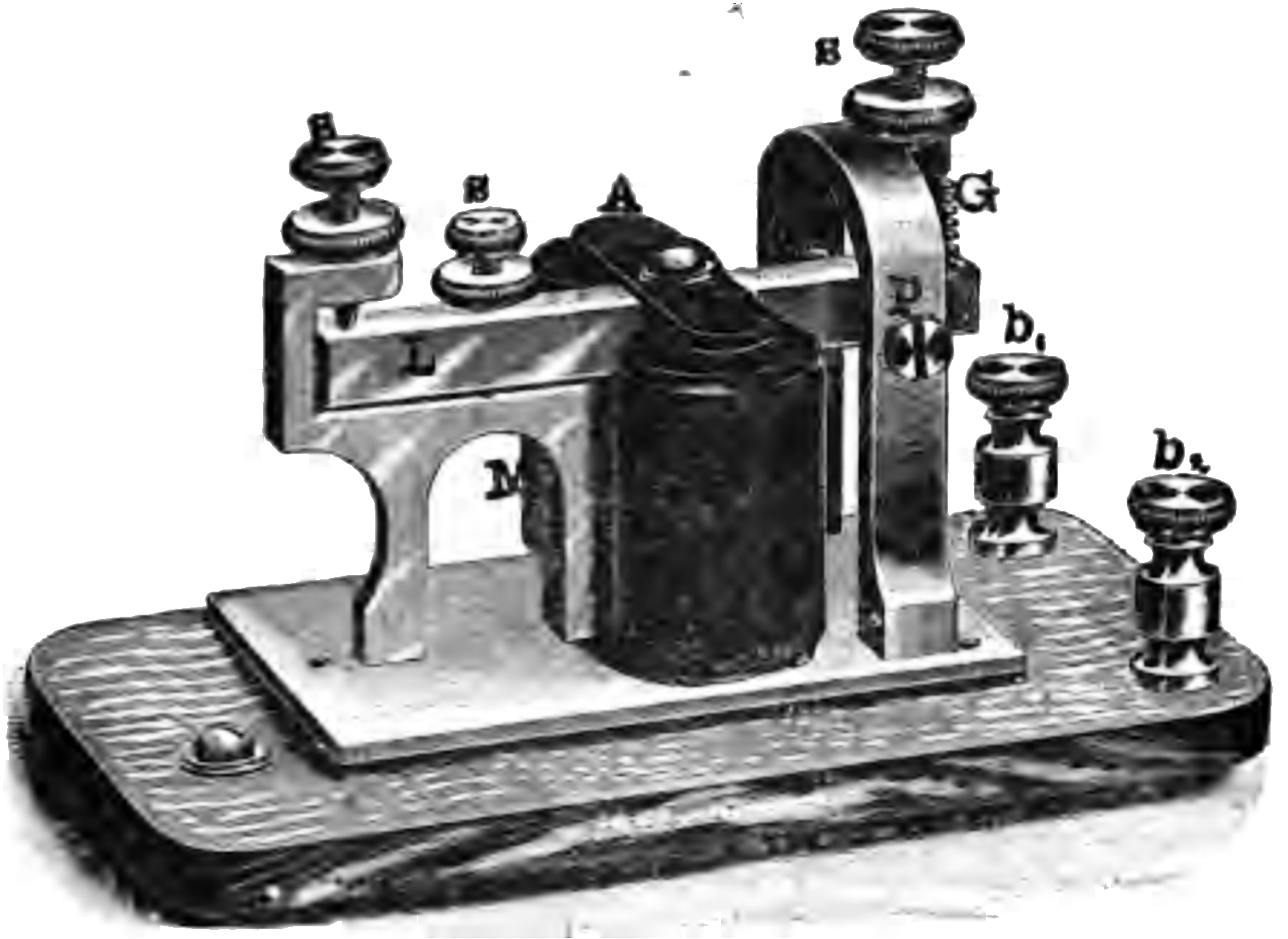
FIG. 54.—TELEGRAPH SOUNDER.
