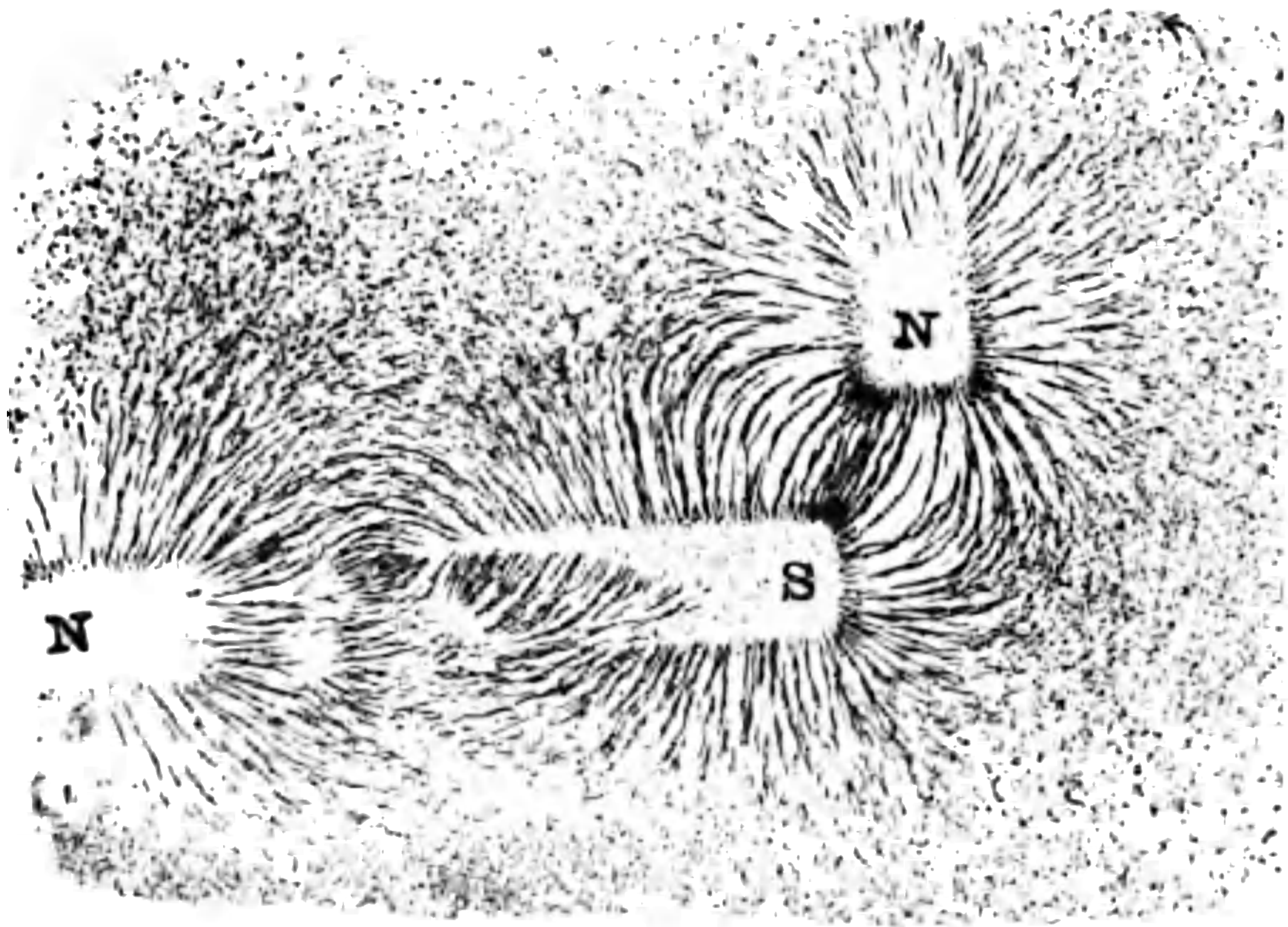
FIG. 23.—FLUX PATHS. UNLIKE POLES AT RIGHT ANGLES.
