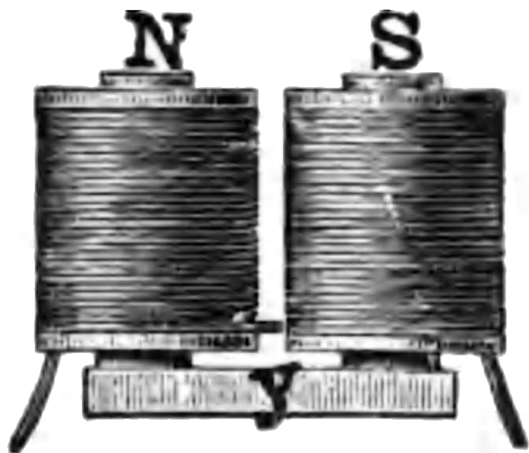
FIG. 43.—ORDINARY FORM OF HORSESHOE ELECTROMAGNET.
