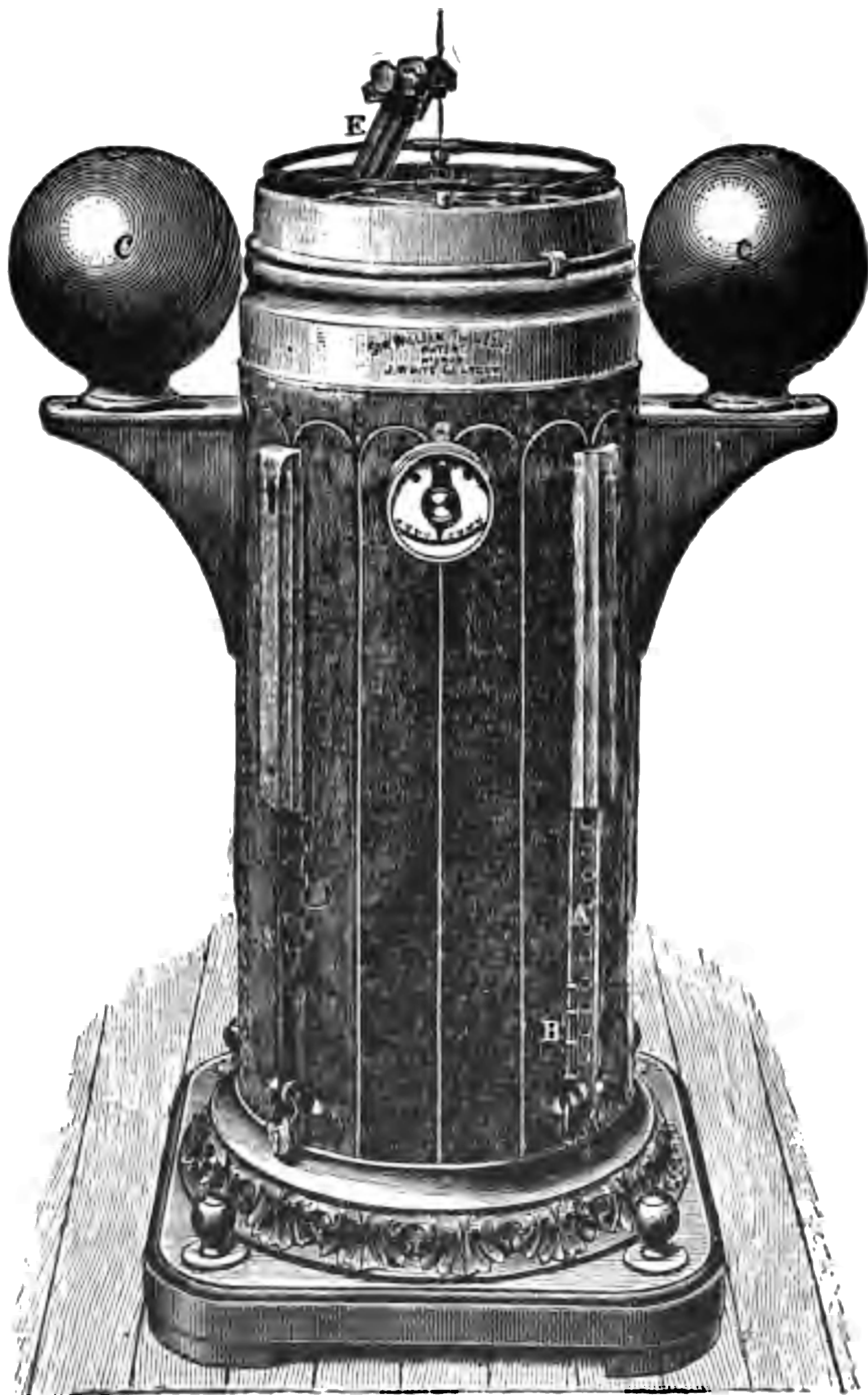
FIG. 93.—THOMPSON'S COMPENSATING BINNACLE.
