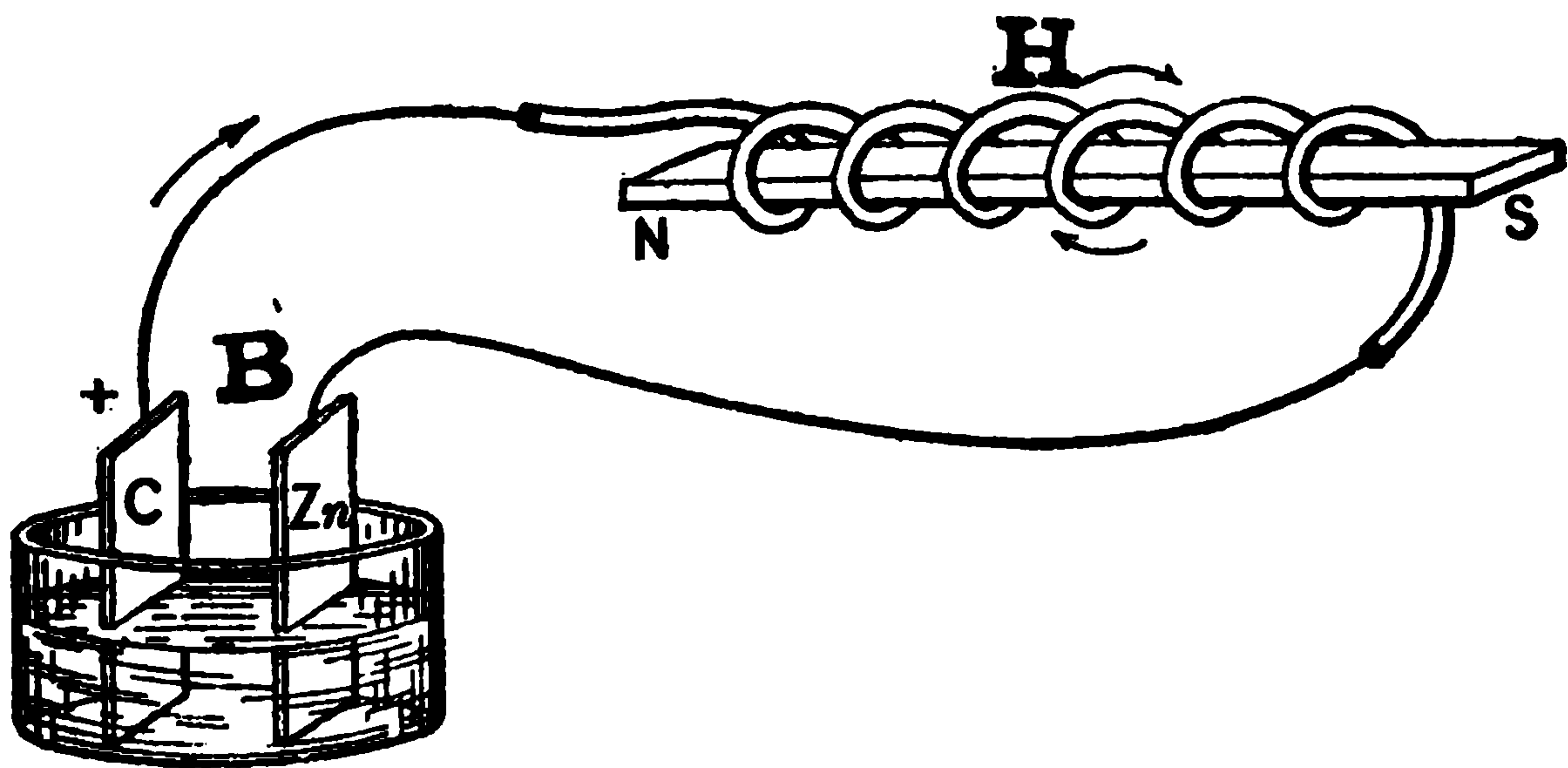
FIG. 18.—VOLTAIC CELL SUPPLYING CURRENT TO A HELIX.
