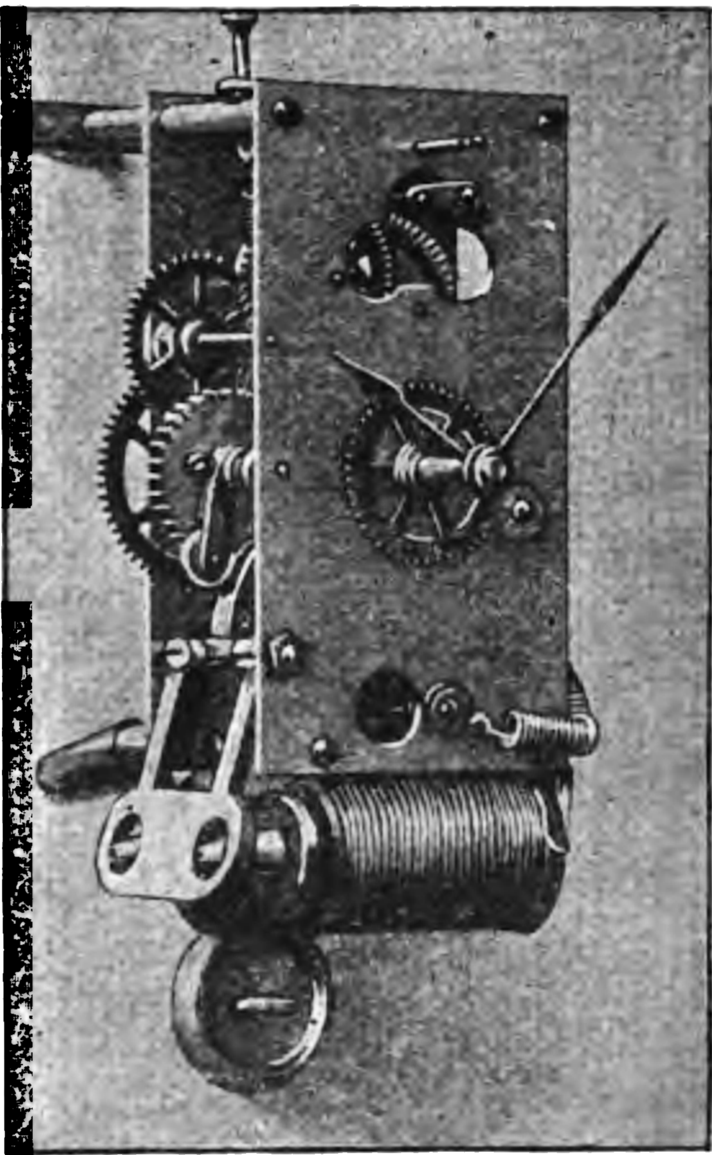
FIG. 63.—SELF-WINDING CLOCK.
