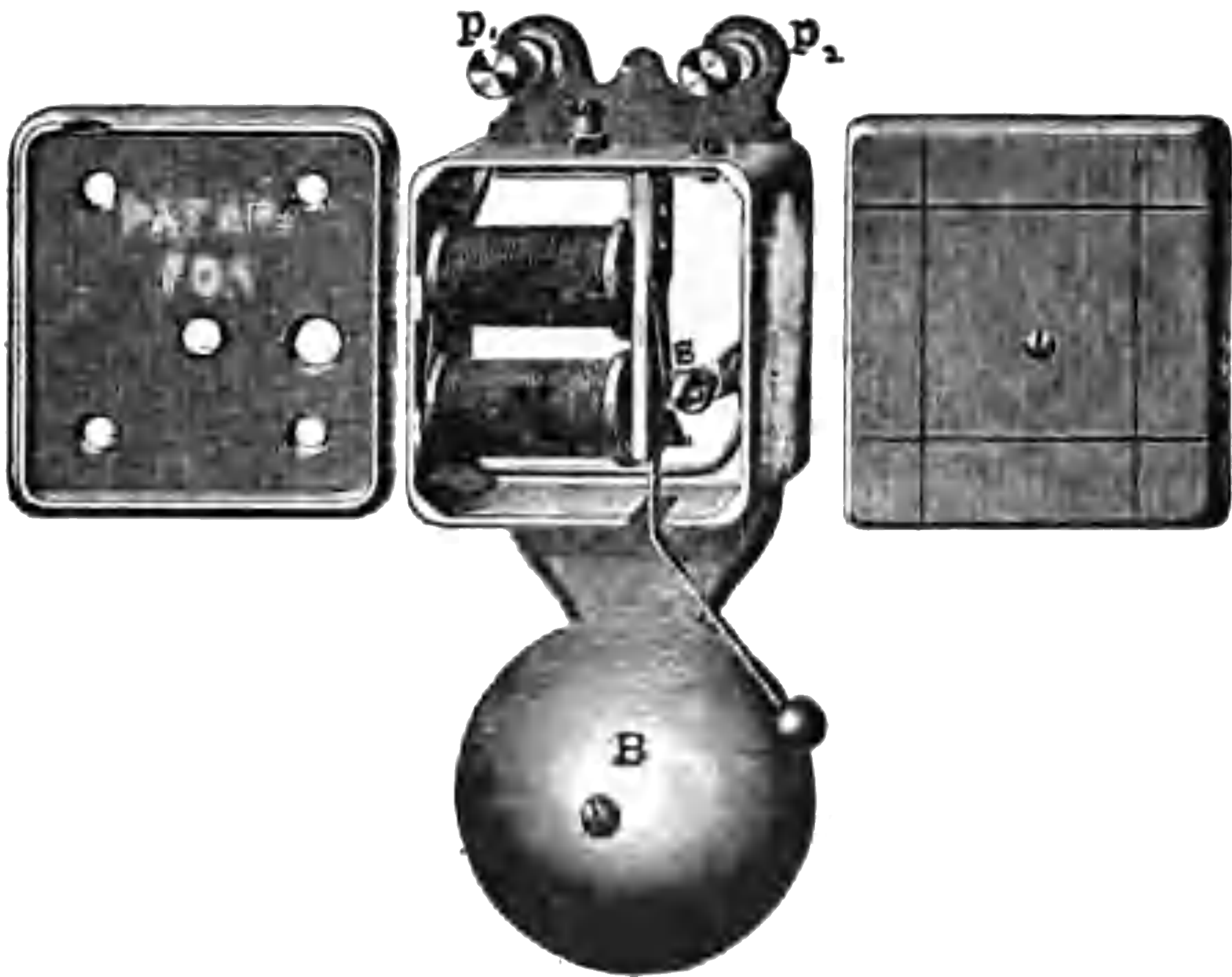
FIG. 57.—ELECTROMAGNETIC BELL.
