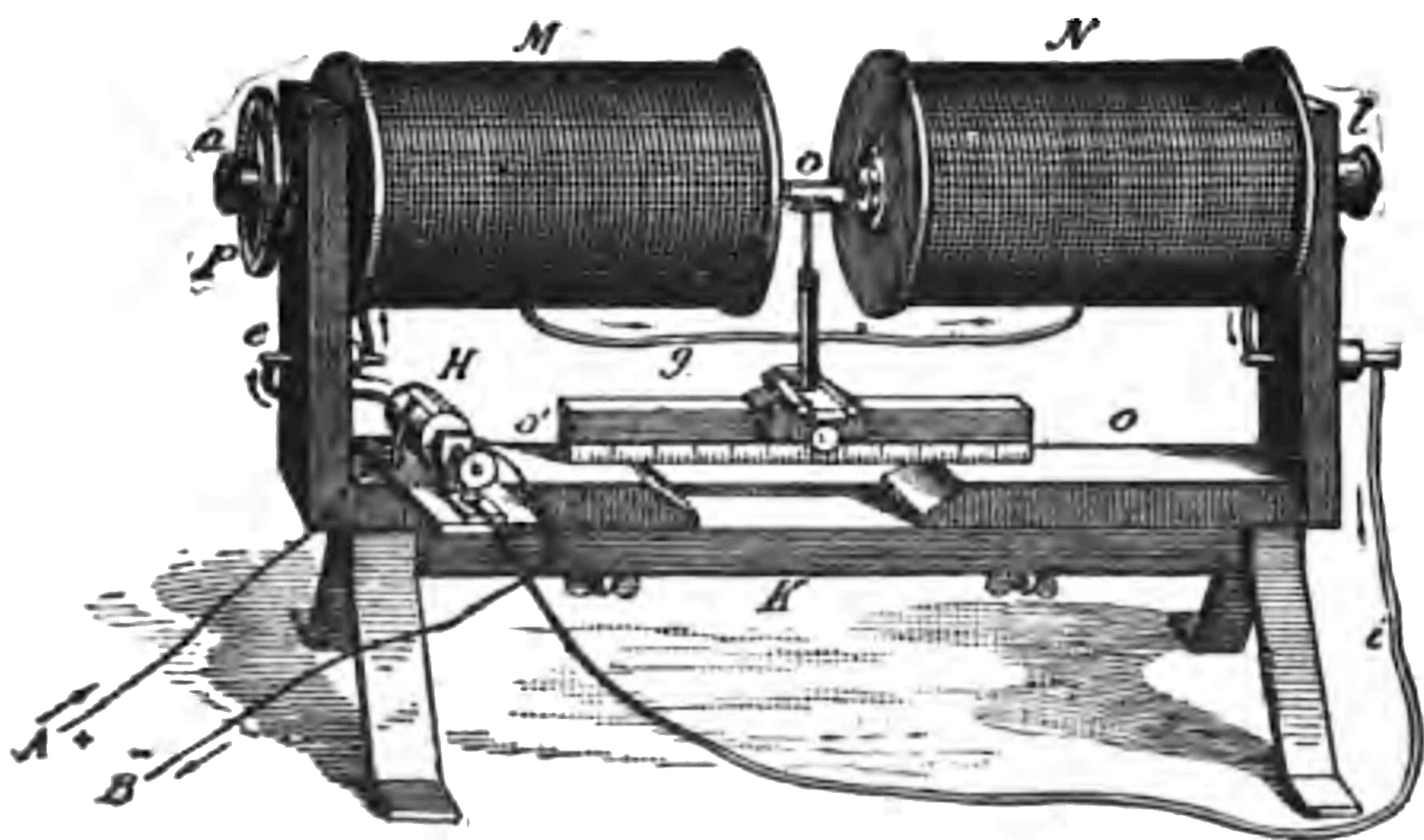
FIG. 79.—APPARATUS FOR PRODUCING MAGNETIC ROTATORY POLARIZATION OF LIGHT.
