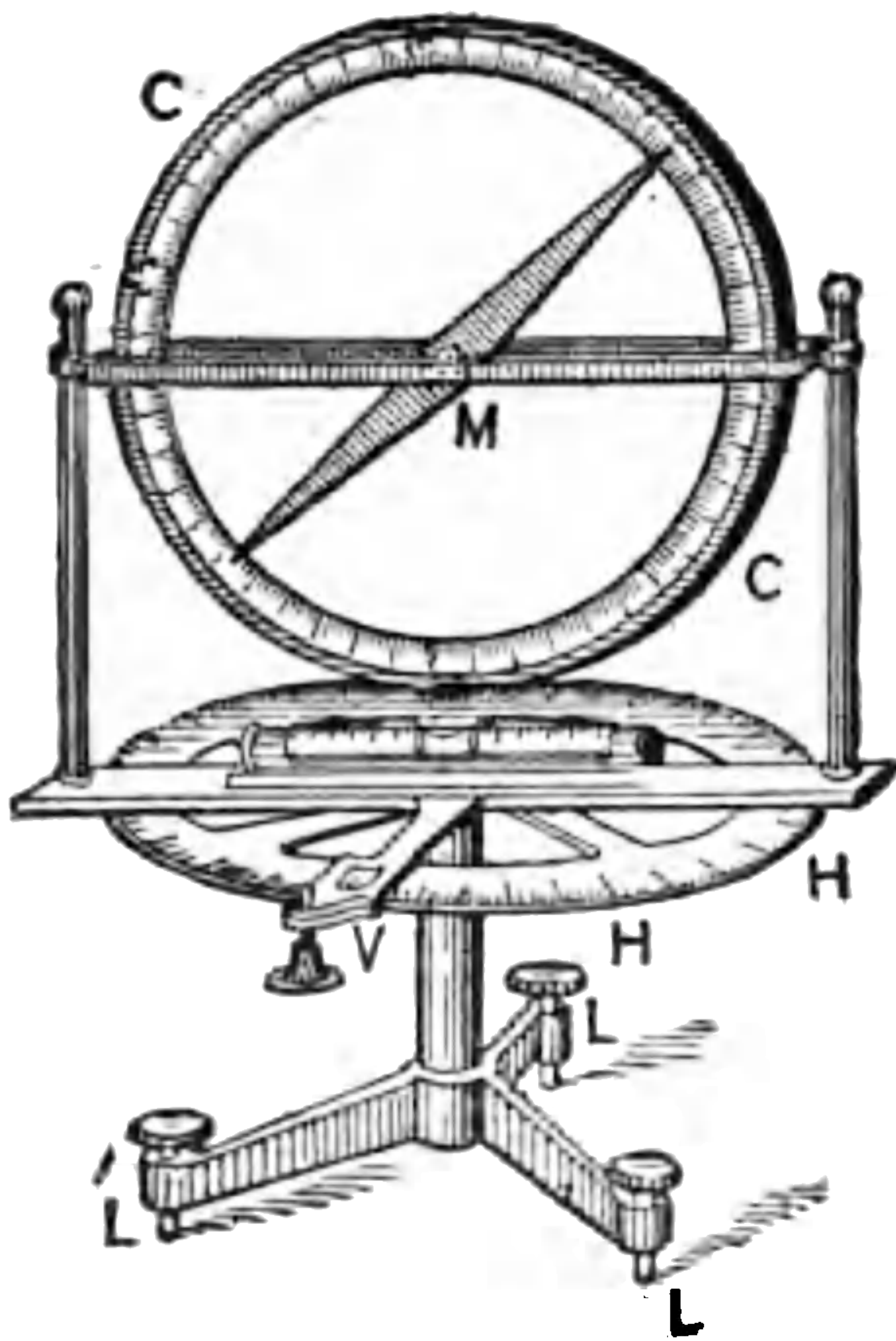
FIG. 84.—DIPPING NEEDLE.
