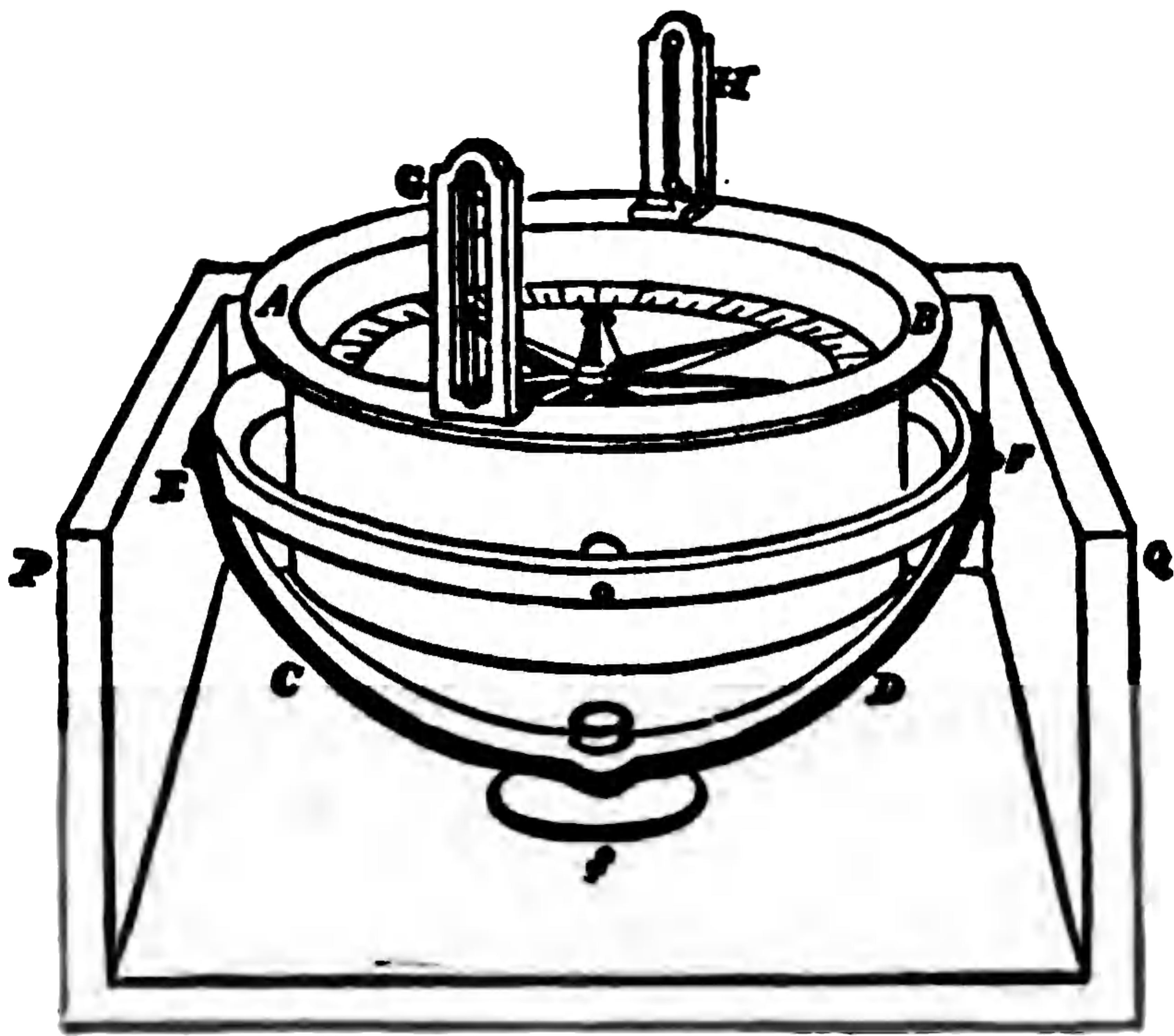
FIG. 92.—MARINER'S COMPASS.
