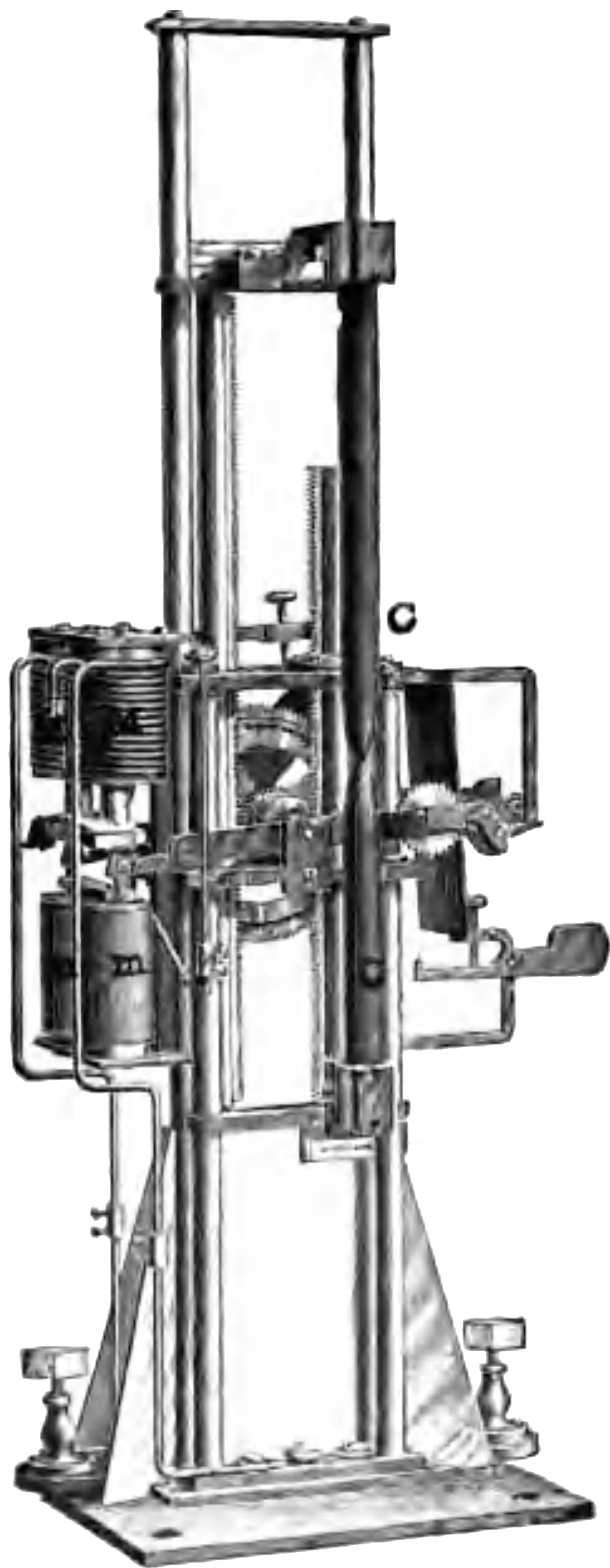
FIG. 60.—ARC-LAMP MECHANISM.
