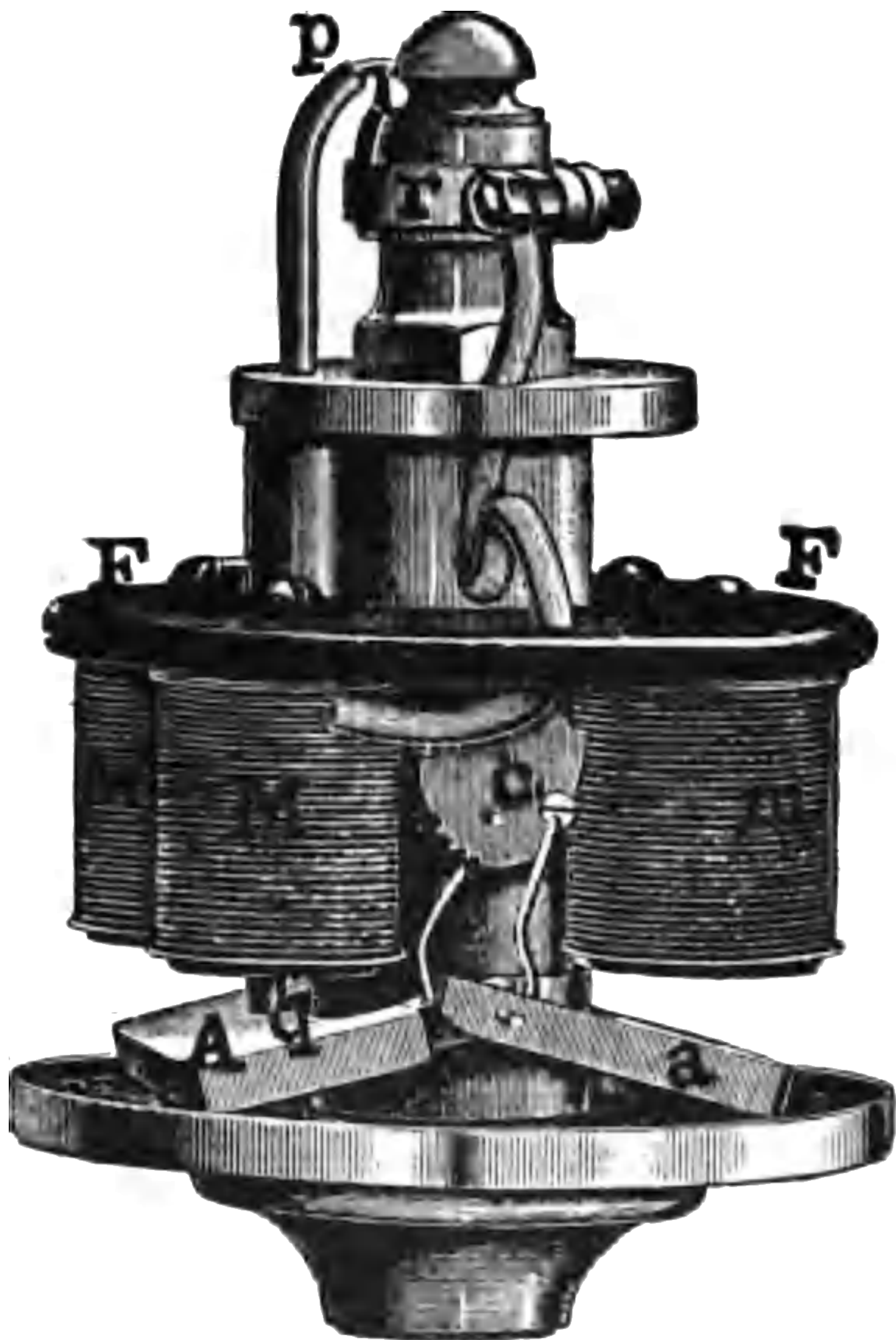
FIG. 61.—ELECTRIC GAS LIGHTING AND EXTINGUISHING MECHANISM.
