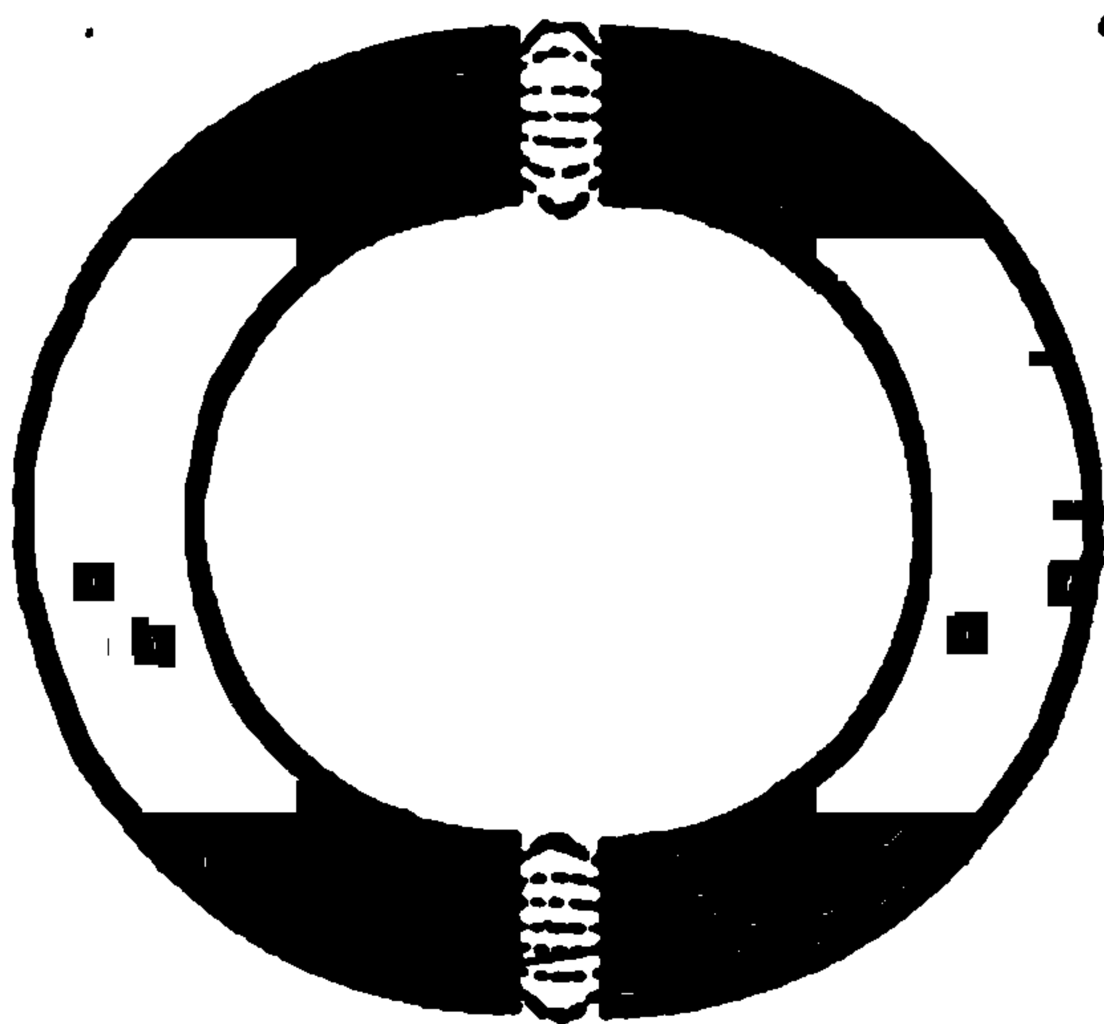
FIG. 17.—AERO-FERRIC MAGNETIC CIRCUIT.
