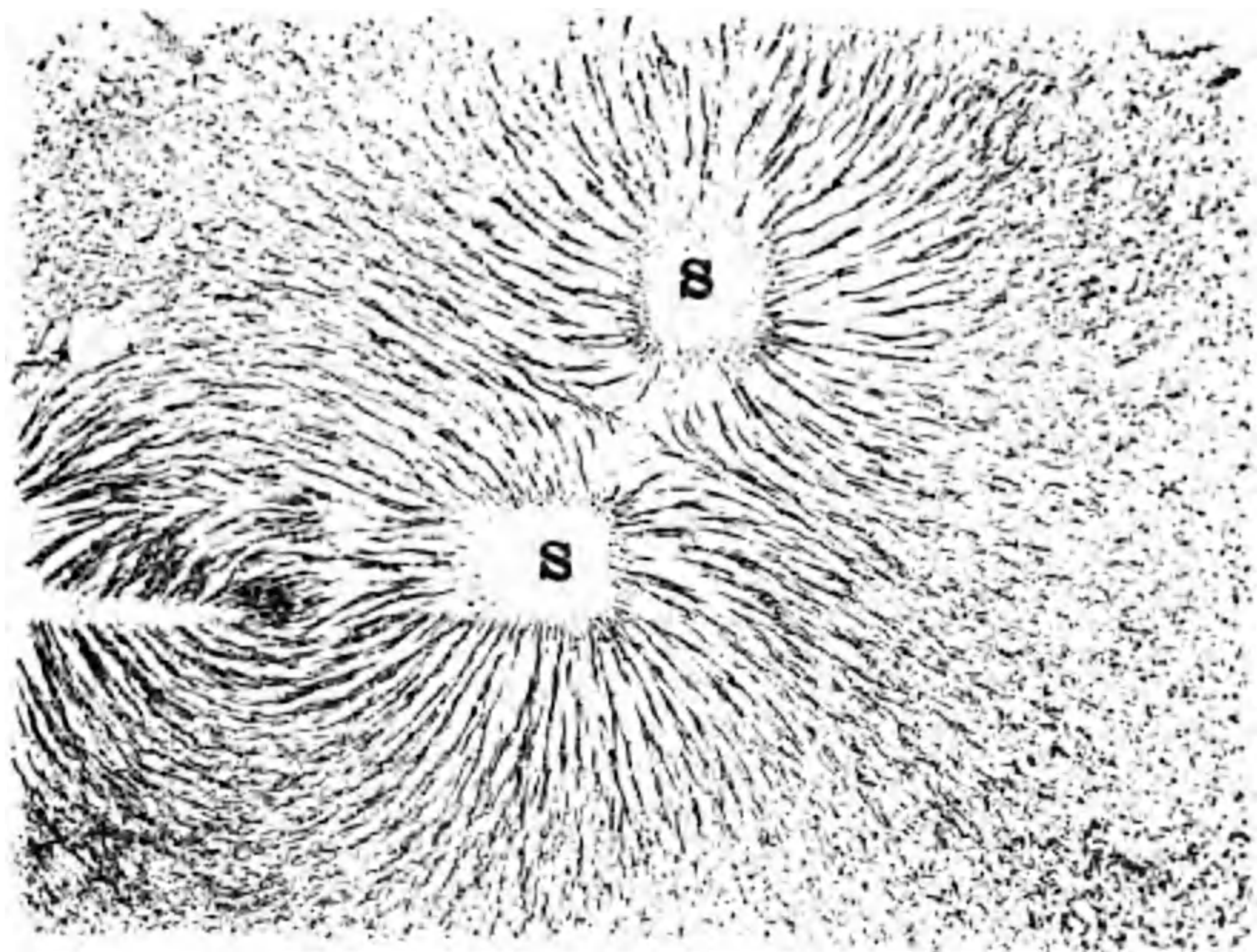
FIG. 24.—FLUX PATHS. LIKE POLES AT RIGHT ANGLES.
