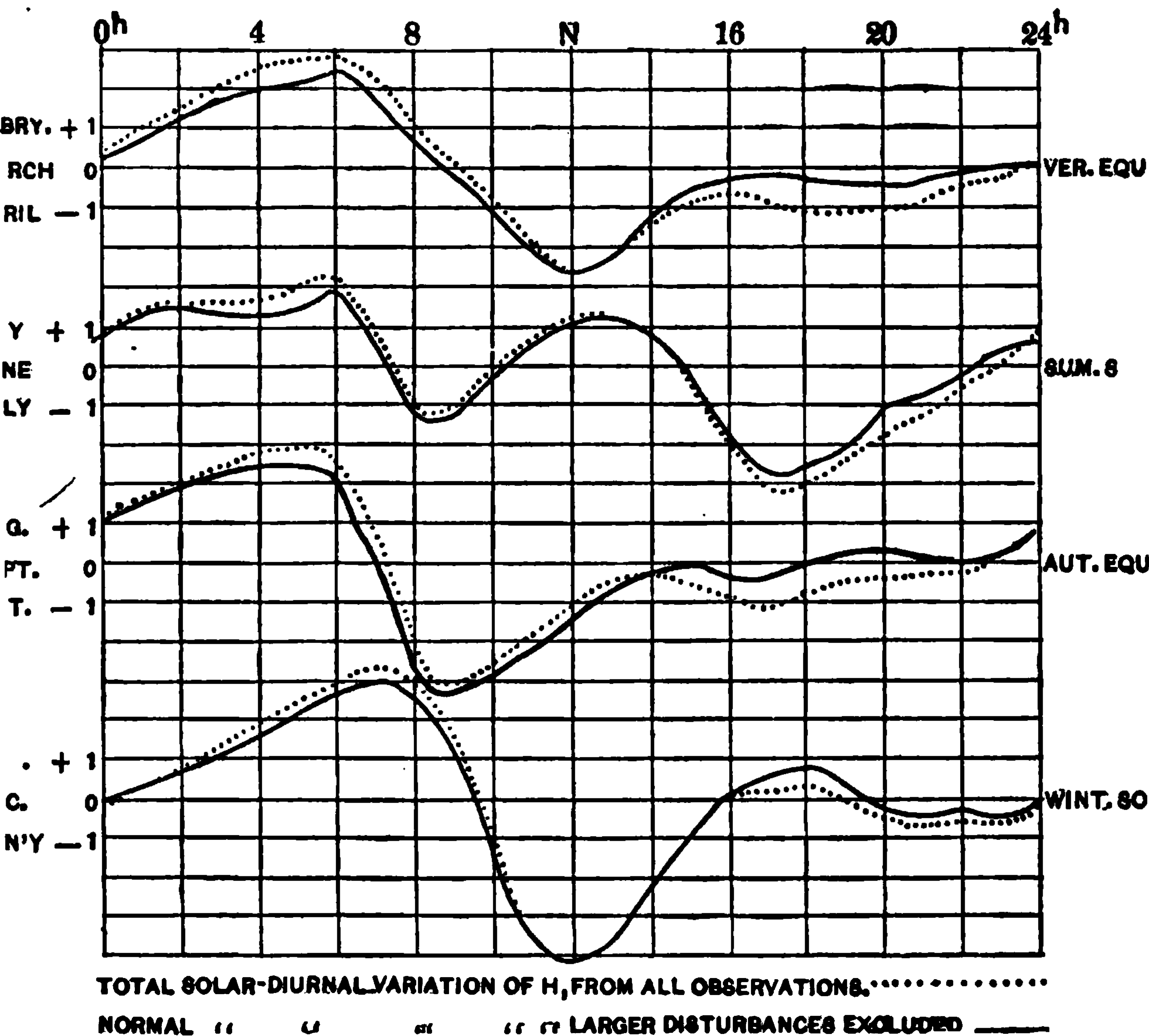
FIG. 89.—CURVES OF TOTAL SOLAR DIURNAL VARIETIES OF THE HORIZONTAL COMPONENT OF MAGNETIC FORCE FOR LOS ANGELES, CAL., COMPILED FROM OBSERVATION IN 1883-1888.
