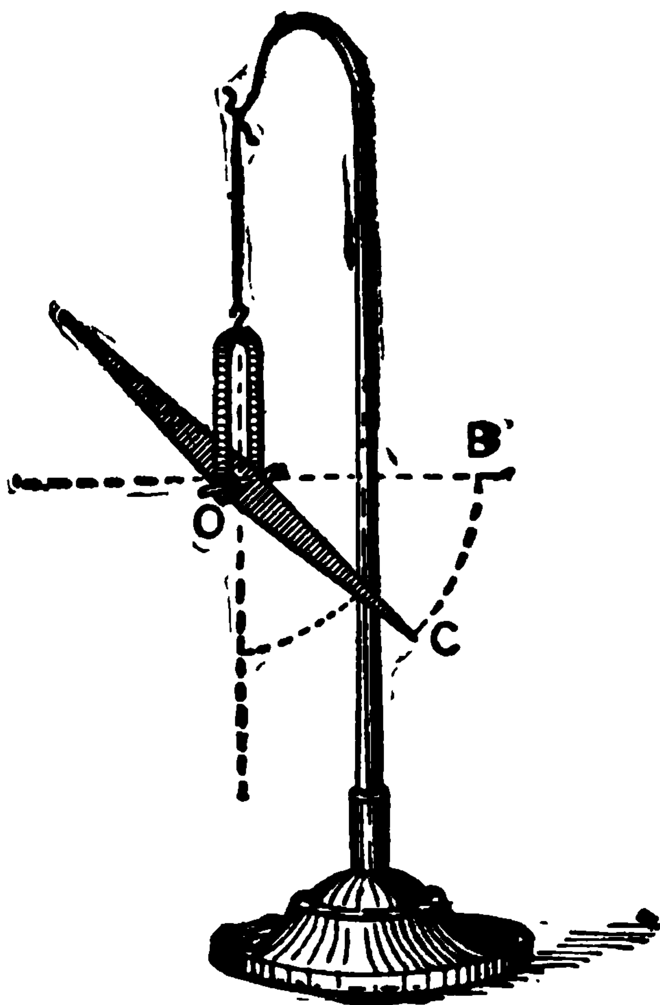
FIG. 82.—DIPPING NEEDLE.
