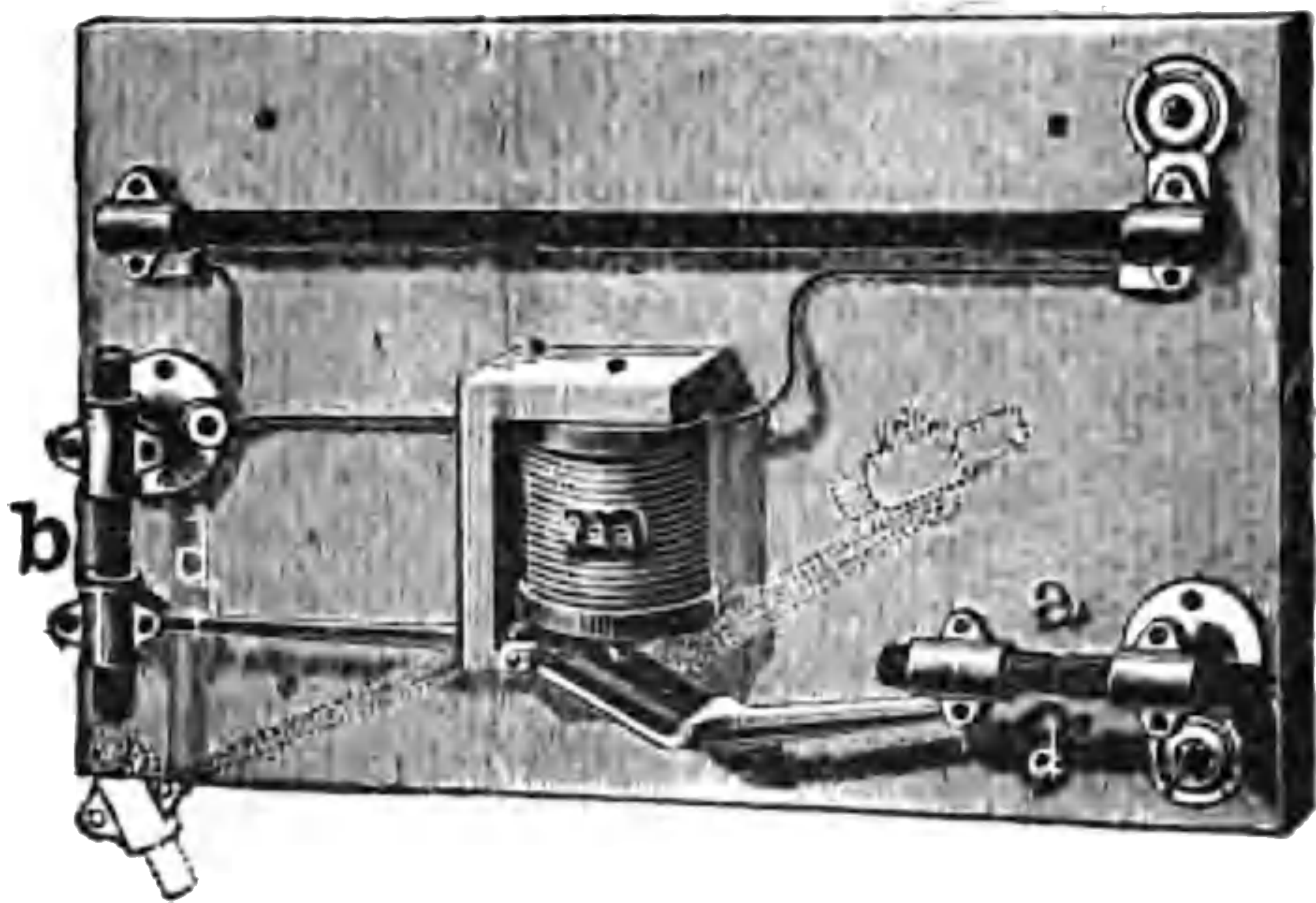
FIG. 65.—ELECTROMAGNETIC LIGHTNING ARRESTER.
