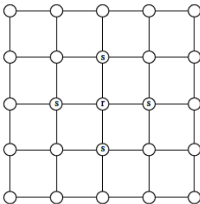
Figure 4.4 Lattice for two-dimensional Ising model. The spins are in the circles. The couplings, K , are the lines. A particular site is labeled with an “ r .” Its nearest neighbors are shown with an “ s .”
