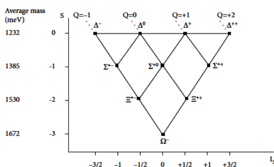
Figure 8.1 A spin-3/2 baryon decuplet
