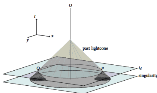
Figure 17.2 This figure illustrates the horizon problem. Lightcones are at 45° but distances are distorted, much like a Mercator projection. Two points p, q on the surface of last scattering t_d , both falling within our past light cone, do not have overlapping light cones.
